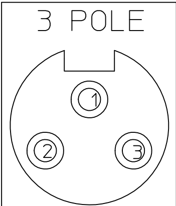
WIDOK OD STRONY DRUTOW VIEW FROM WIRES SIDE
