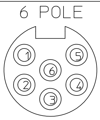
WIDOK OD STRONY DRUTOW VIEW FROM WIRES SIDE
