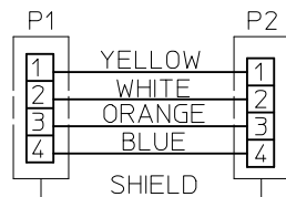
WIRING DIAGRAM
