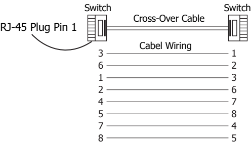
RJ-45 8-wiring Cross-Over definition
