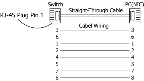
RJ-45 8-wiring normal definition
