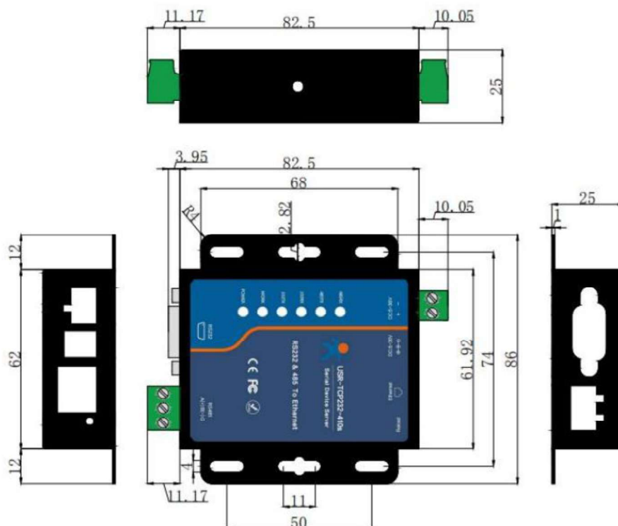
Fig1. Dimension of TCP232-410s
