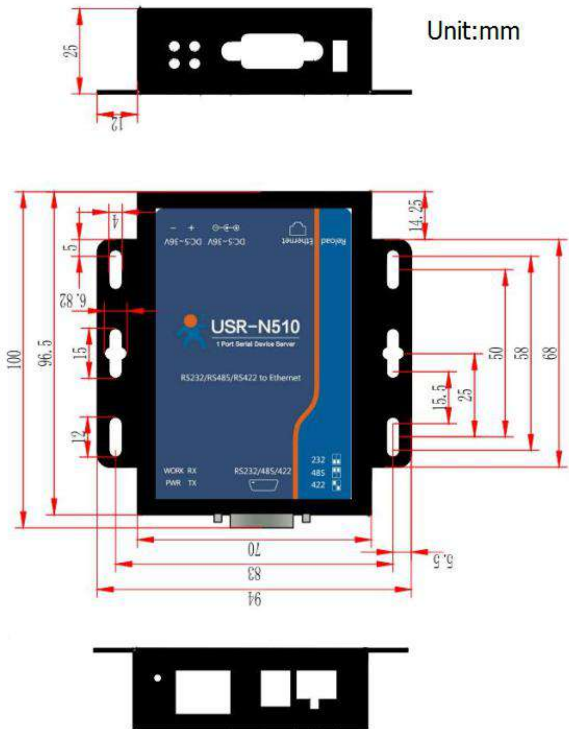
Figure 7 Hardware dimensions
