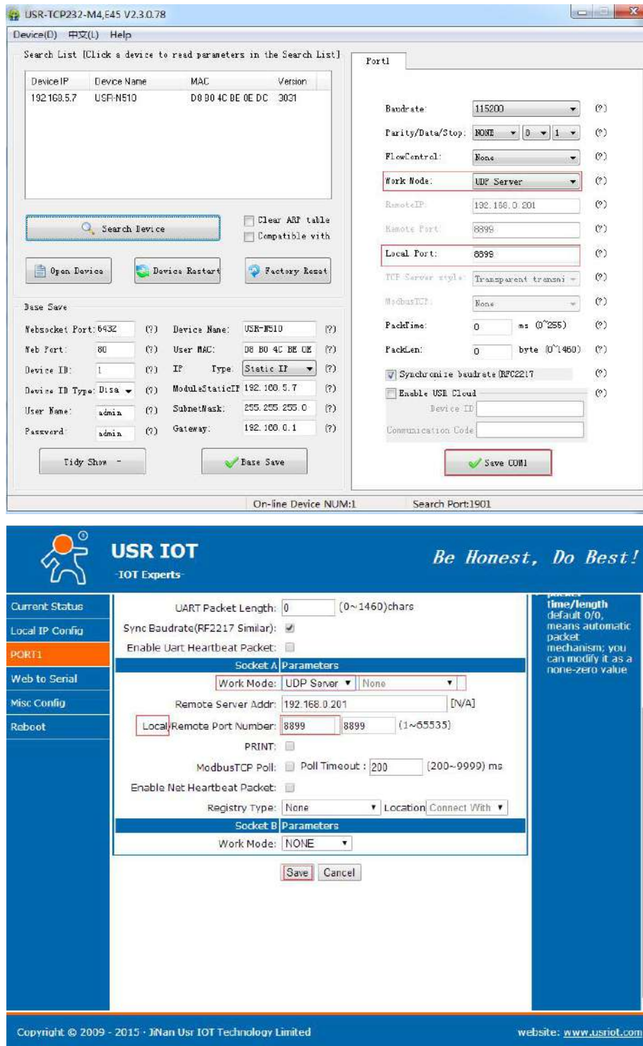
Figure 17 UDP Server
