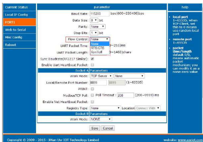
Figure 20 Flow Control
