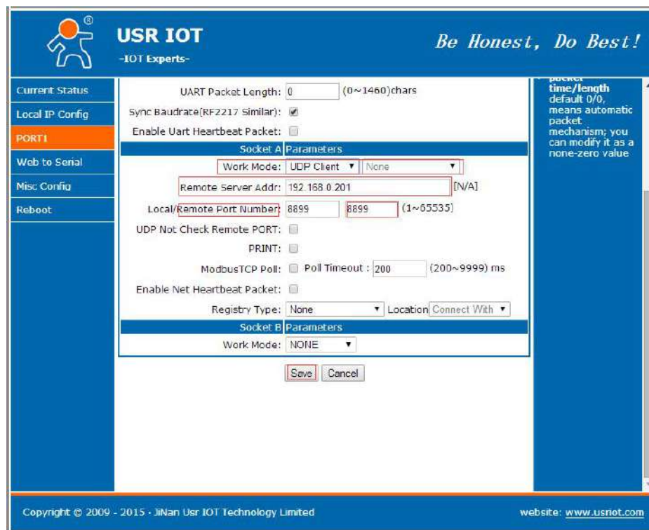
Figure 16 UDP Client
