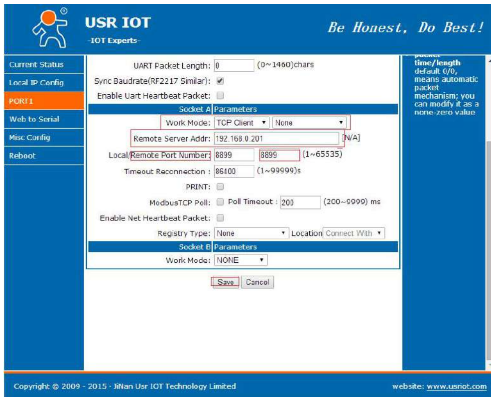
Figure 14 TCP Client
