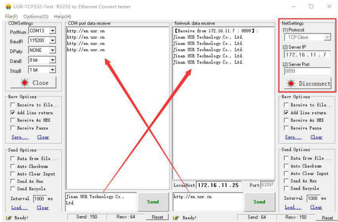
Figure 3 data transmission
