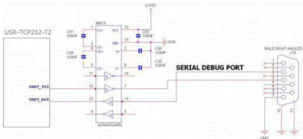
Diagram 3.2.3-1 UART Interface Design
