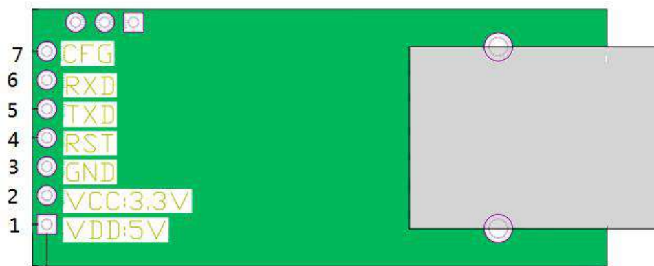
Diagram 3.1.1-1 T2 Interface Definition
