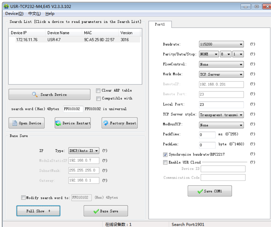
Diagram 5-5 Software setup parameters - port configuration
