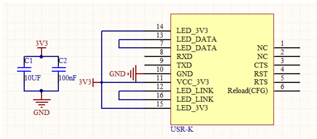
Diagram 4-5 connection diagram
