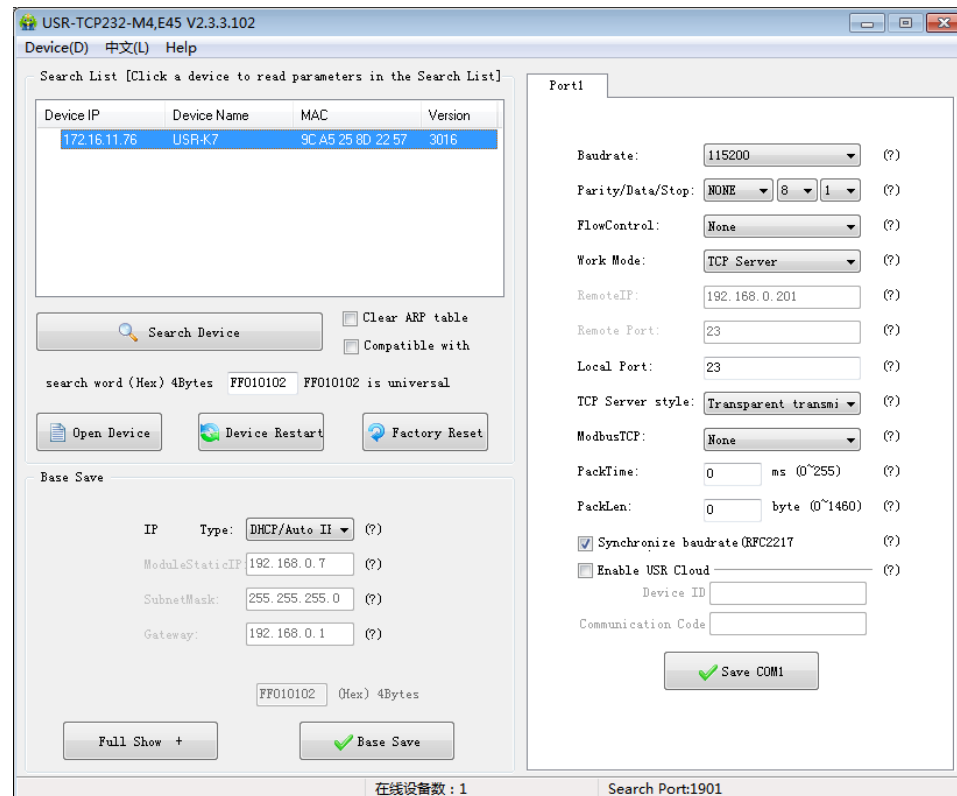
Diagram 5-1 Software setup parameters - search
